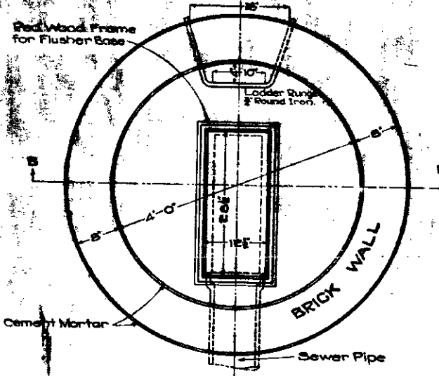
FLOOR PLAN Scale 1/4"
