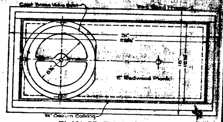
PLAN OF FLUSHER BASE Scale 1/2"
