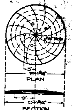
SECTION CAST IRON COVER Scale 1/4"
